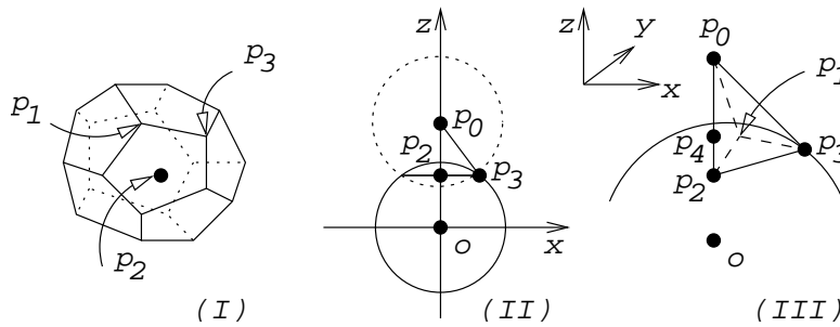
Figure 4. Illustration for the computation of \delta_3(dc) .
