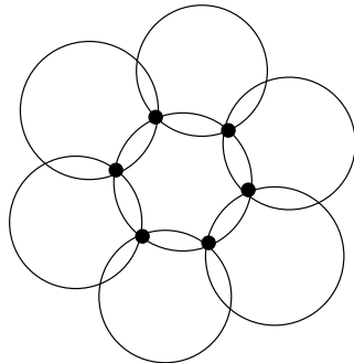
Figure 1. A regular hexagonal covering.
