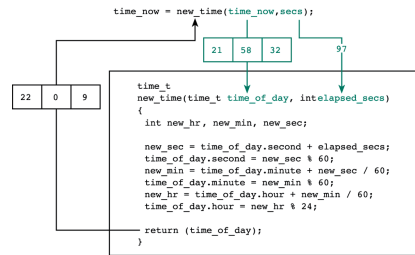
Figure 11.8 Structured Values as a Function Input Argument and as a Function Result
