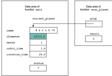
Figure 11.5 Data Areas of main and scan_planet during Execution of status = scan_planet (&current_planet);
