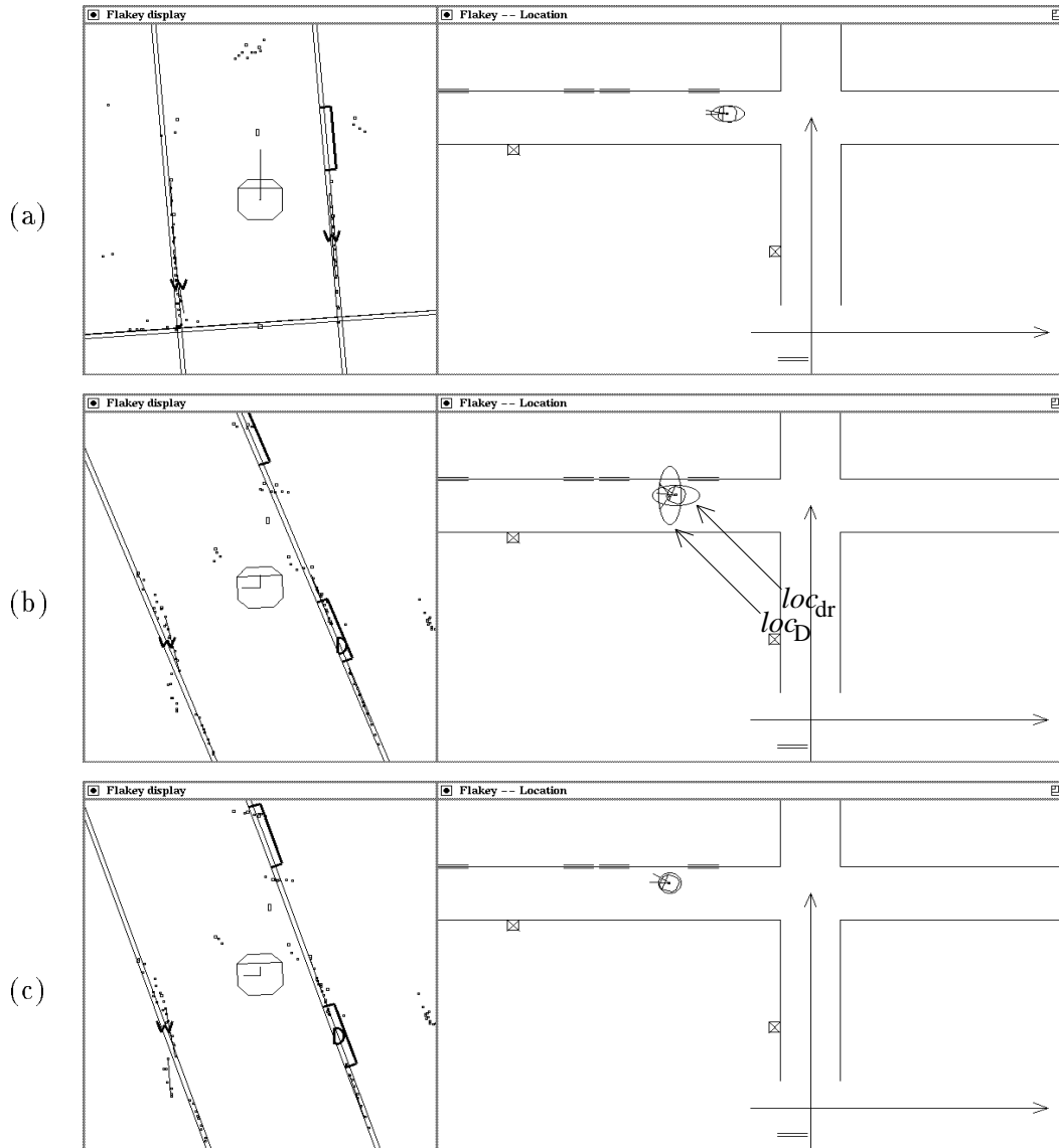
Figure 13: Fuzzy self-localization. Left: the robot's internal view of its surroundings. Right: the robot's map of the environment, with (a) initial location hypothesis H_t ; (b) dead reckoning and door localizers; (c) updated hypothesis H_{t+1} .
