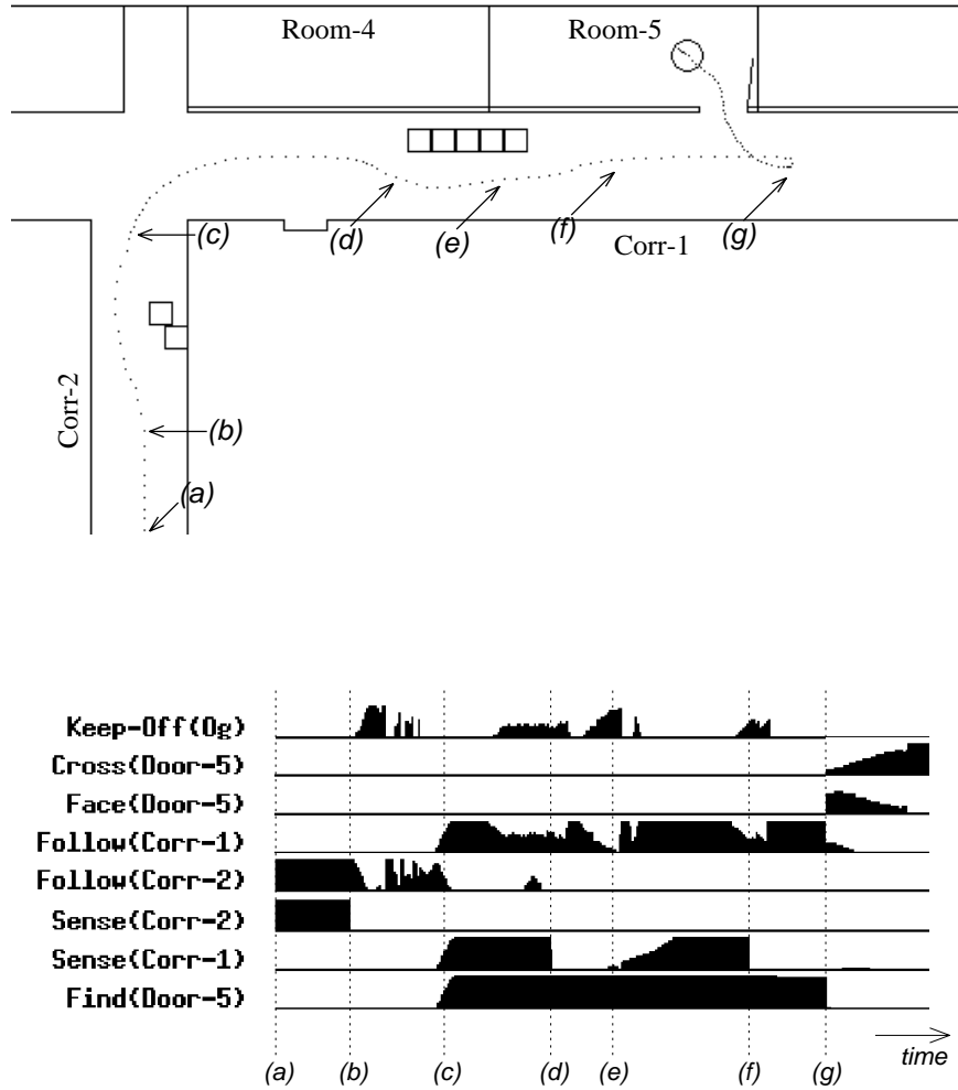
Figure 10: A run of the plan in Figure 9 (top), and the corresponding evolution over time of the activation of the behaviors (bottom).
