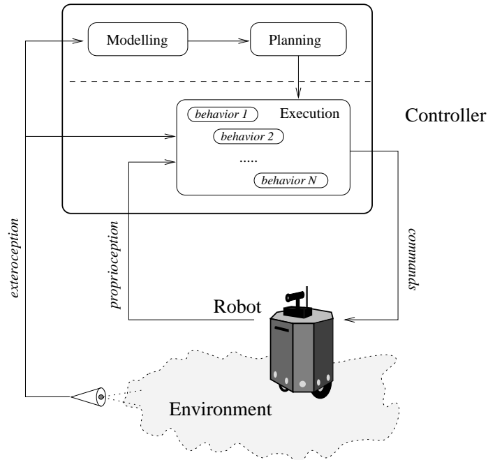
Figure 3: Hybrid architecture. The lower layer uses perception to dynamically adapt plan execution to the environmental contingencies. Complexity in this layer is managed by a divide et impera strategy.
