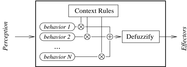
Figure 7: A hierarchical fuzzy controller that implements Context-Dependent Blending.
