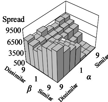
(a) 2-500 test problem.
