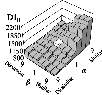
(b) 3-500 test problem.
