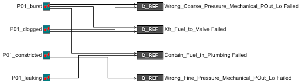
Figure 9. Part of the good Pump and Valve TFGP model. The model was used to diagnosis the ground truth and to simulate maintenance events that would discover the true fault in the bad model.
